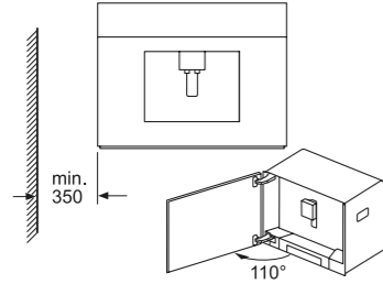
left corner installation
