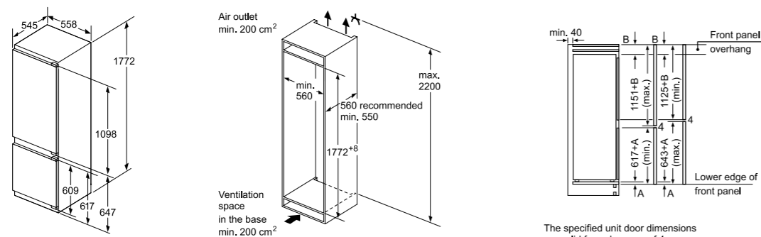
The specified unit door dimensions are valid for a door gap of 4 mm.
